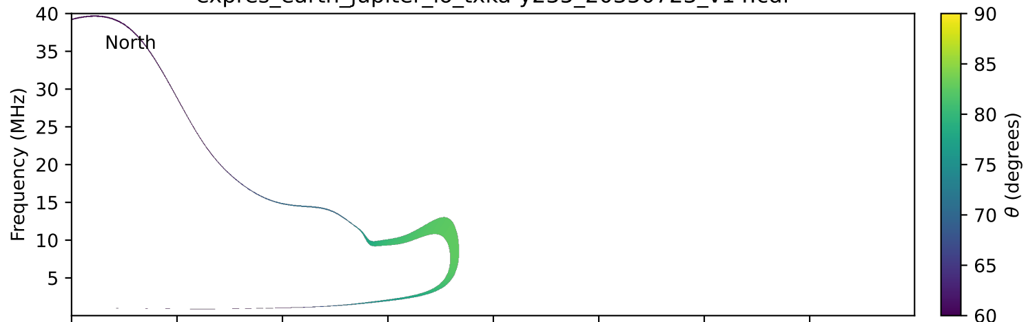
expres_earth_jupiter_io_txka-y235_20350723_v14.cdf
