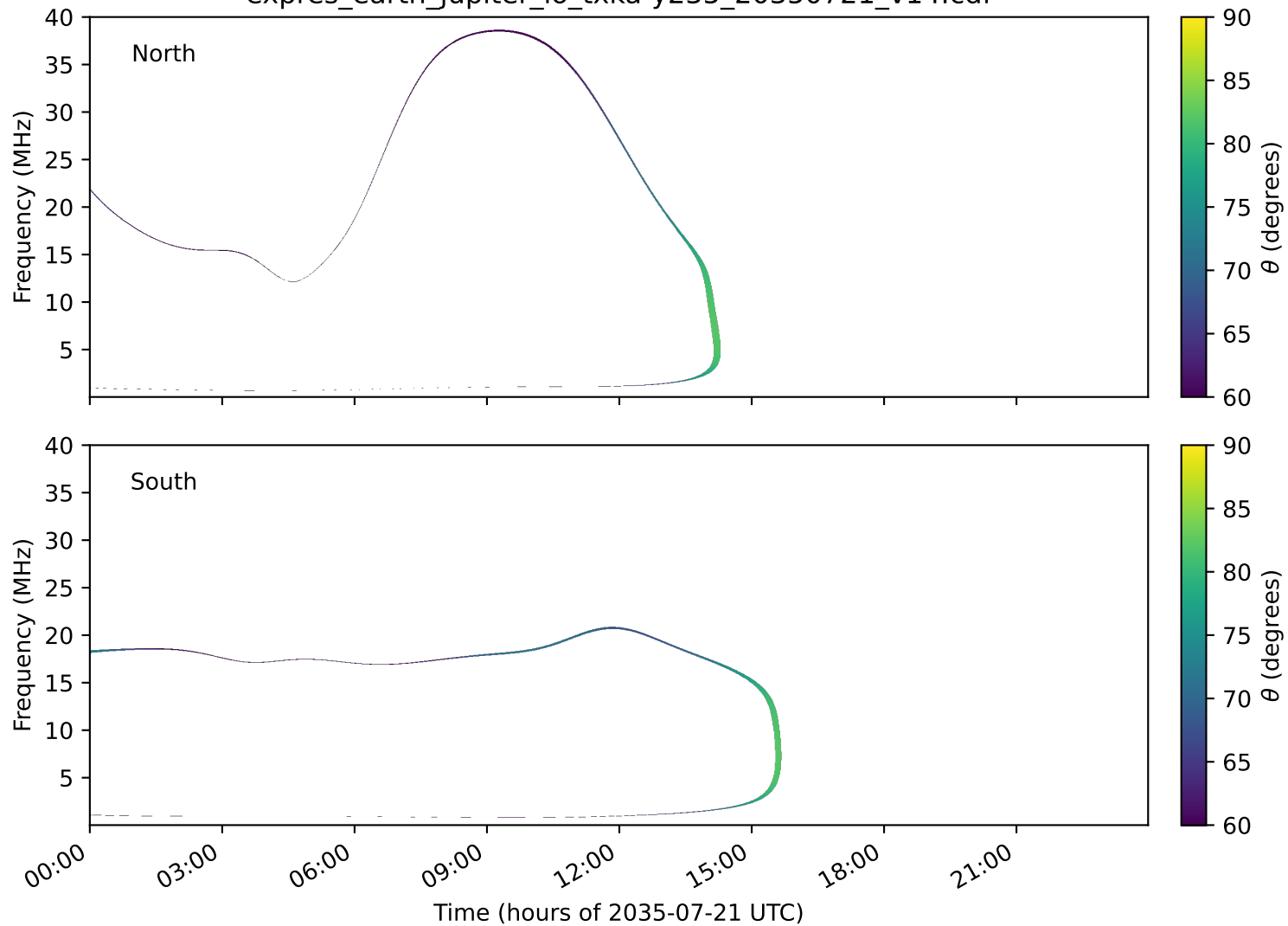
expres_earth_jupiter_io_txka-y235_20350721_v14.cdf
