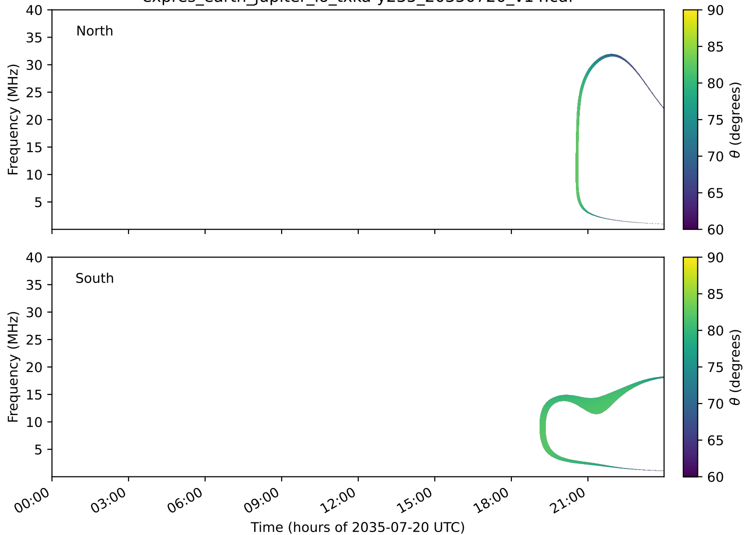
expres_earth_jupiter_io_txka-y235_20350720_v14.cdf
