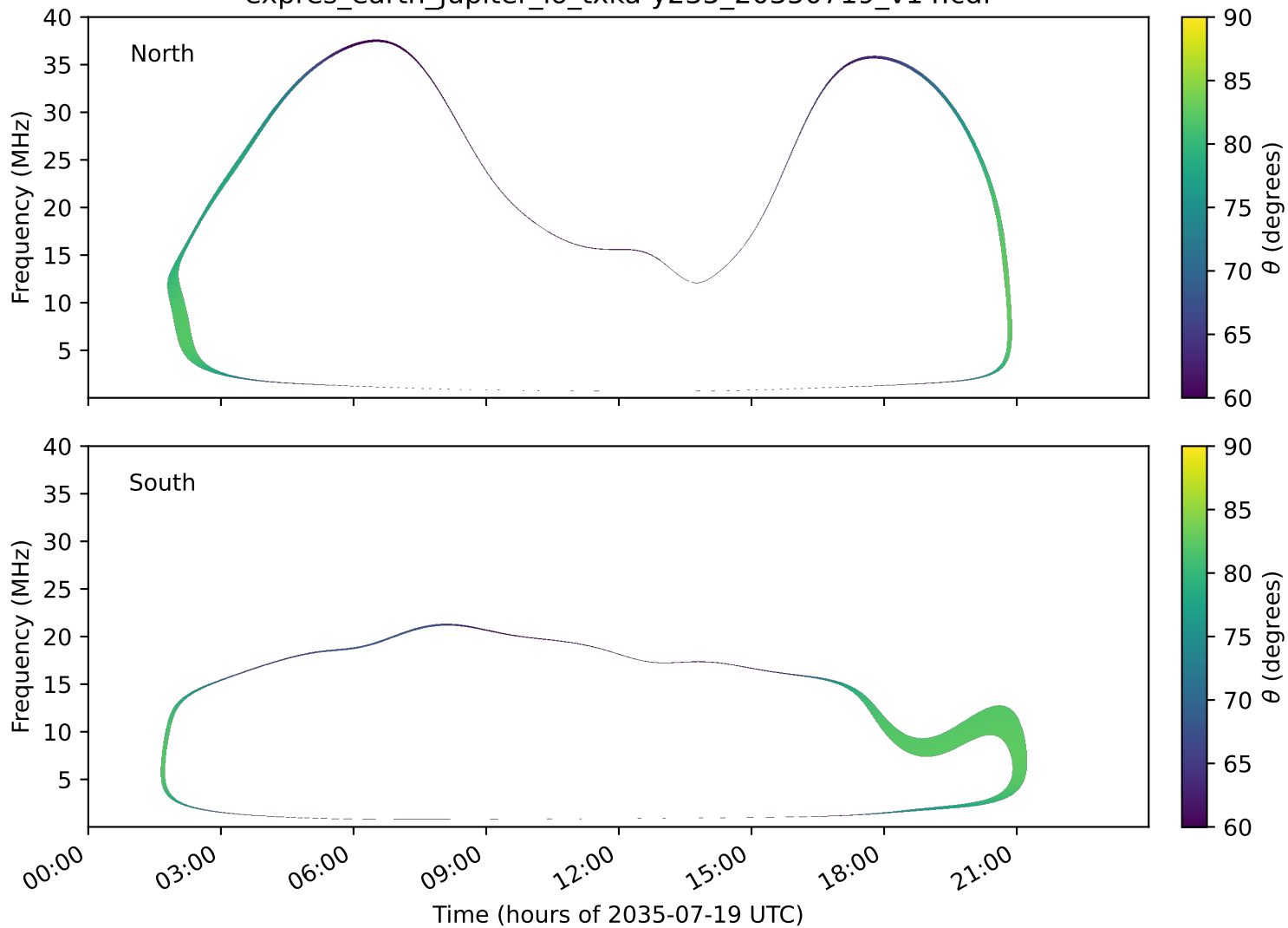
expres_earth_jupiter_io_txka-y235_20350719_v14.cdf
