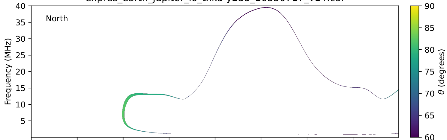
expres_earth_jupiter_io_txka-y235_20350717_v14.cdf
