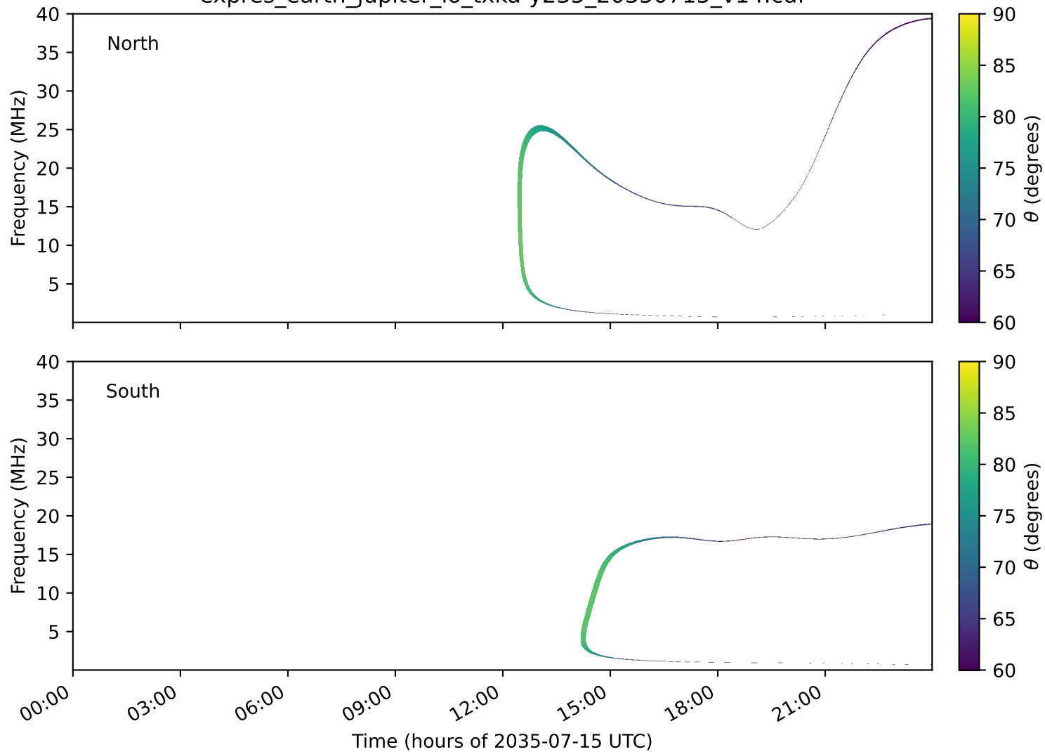
expres_earth_jupiter_io_txka-y235_20350715_v14.cdf
