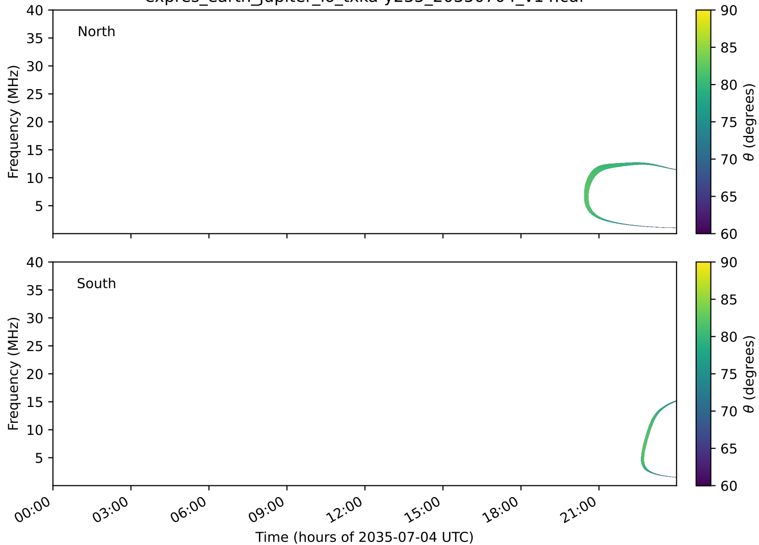
expres_earth_jupiter_io_txka-y235_20350704_v14.cdf
