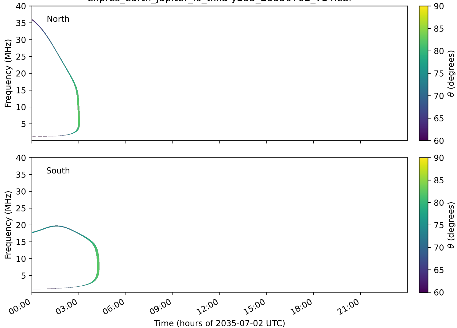
expres_earth_jupiter_io_txka-y235_20350702_v14.cdf
