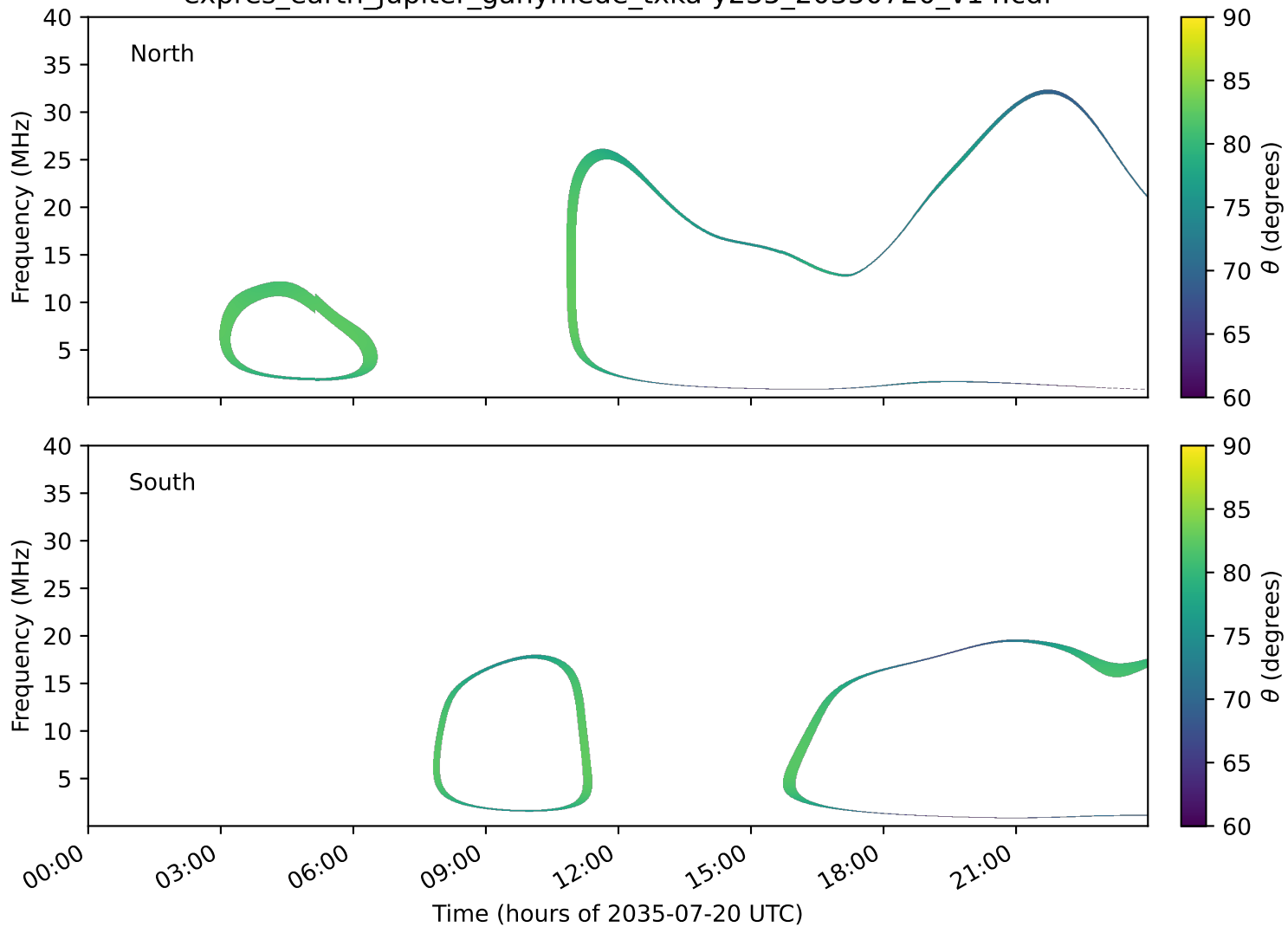
expres_earth_jupiter_ganymede_txka-y235_20350720_v14.cdf
