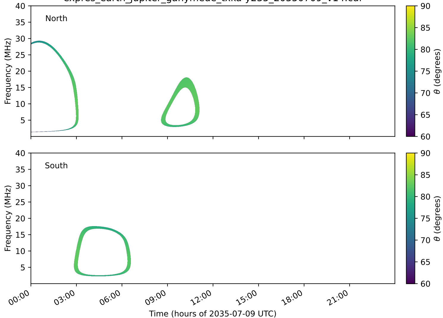
expres_earth_jupiter_ganymede_txka-y235_20350709_v14.cdf
