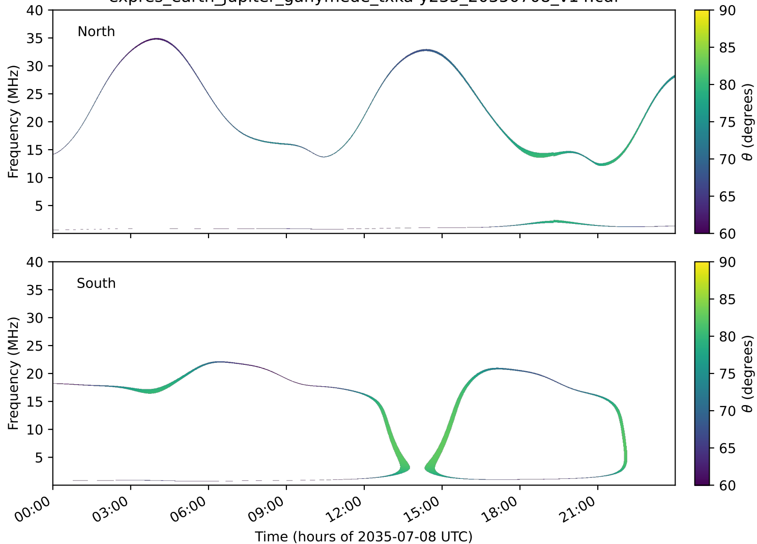
expres_earth_jupiter_ganymede_txka-y235_20350708_v14.cdf
