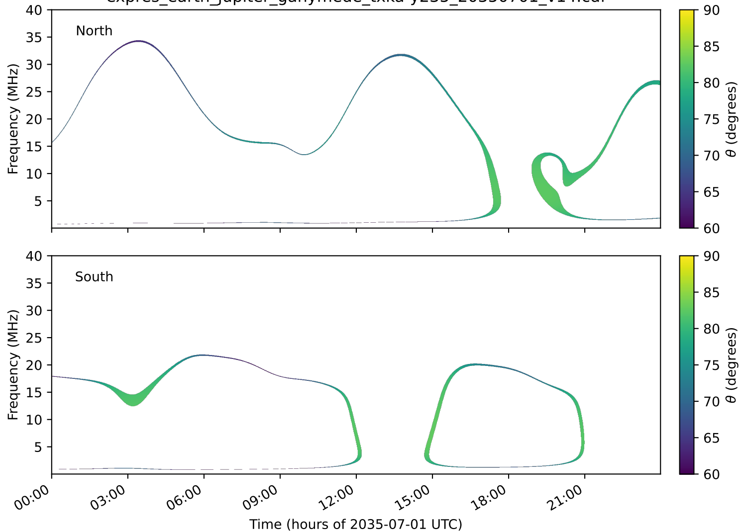
expres_earth_jupiter_ganymede_txka-y235_20350701_v14.cdf
