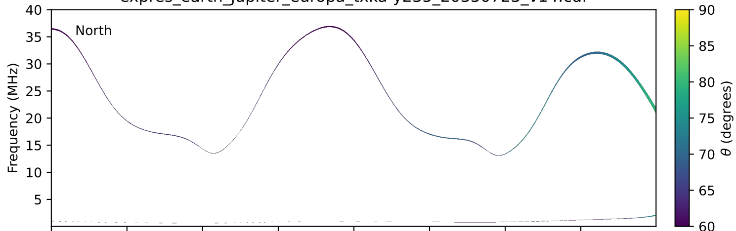
expres_earth_jupiter_europa_txka-y235_20350723_v14.cdf
