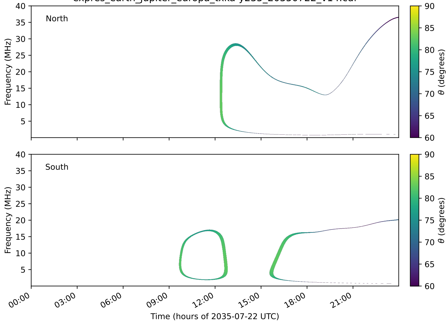
expres_earth_jupiter_europa_txka-y235_20350722_v14.cdf
