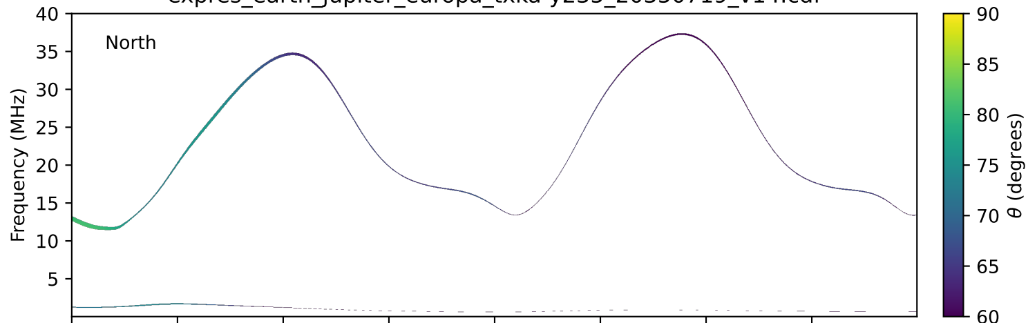
expres_earth_jupiter_europa_txka-y235_20350719_v14.cdf
