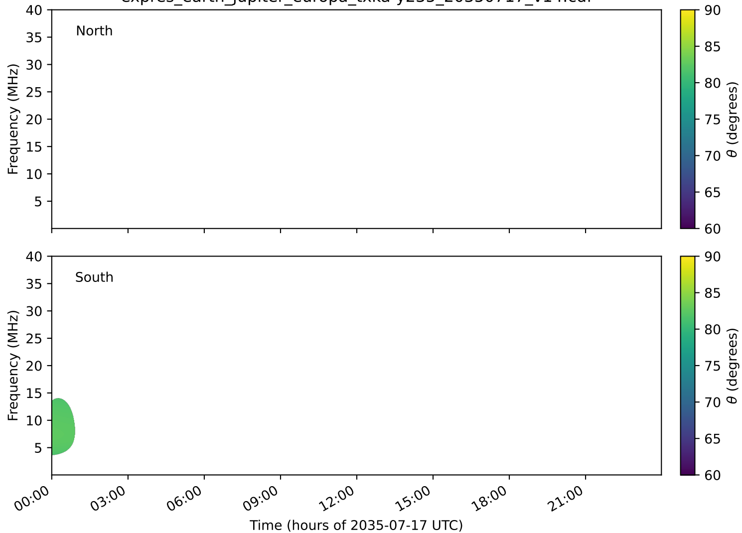
expres_earth_jupiter_europa_txka-y235_20350717_v14.cdf
