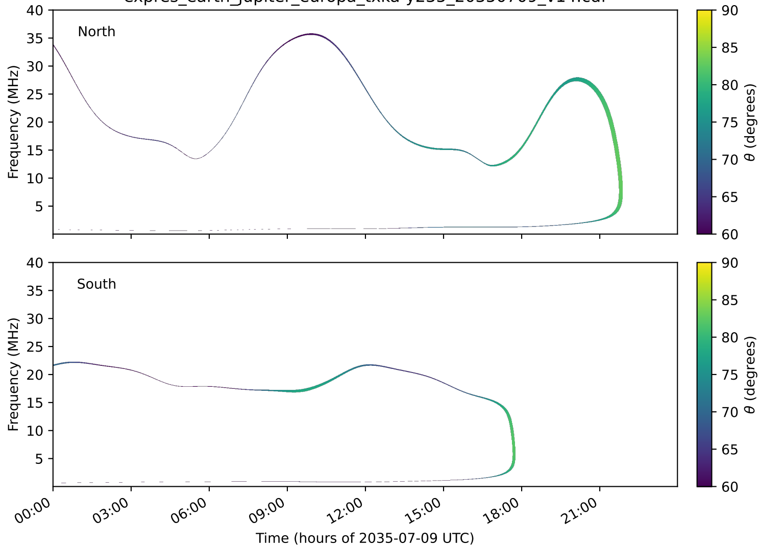
expres_earth_jupiter_europa_txka-y235_20350709_v14.cdf
