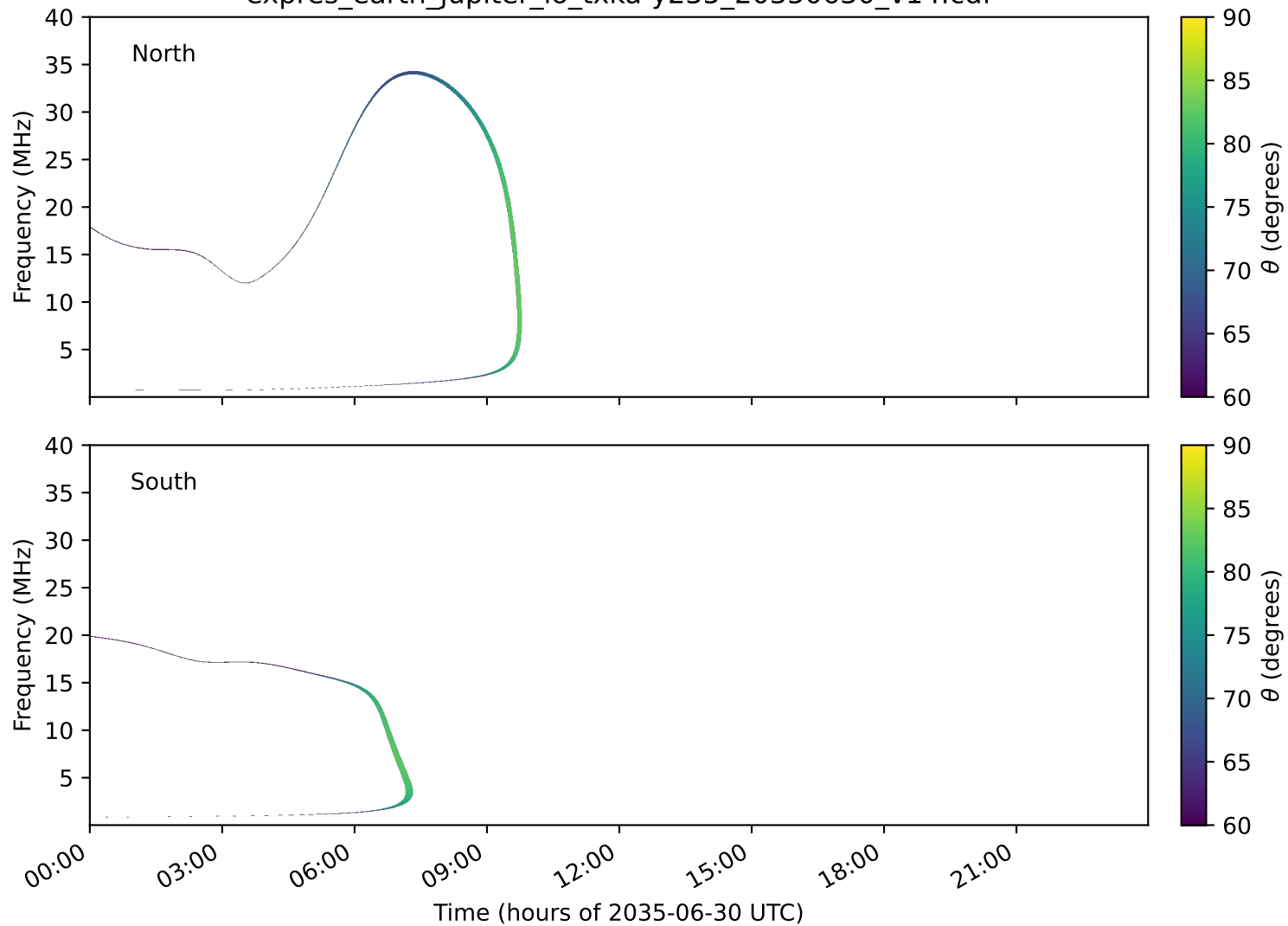
expres_earth_jupiter_io_txka-y235_20350630_v14.cdf
