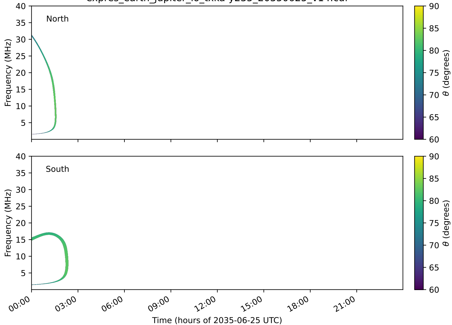
expres_earth_jupiter_io_txka-y235_20350625_v14.cdf
