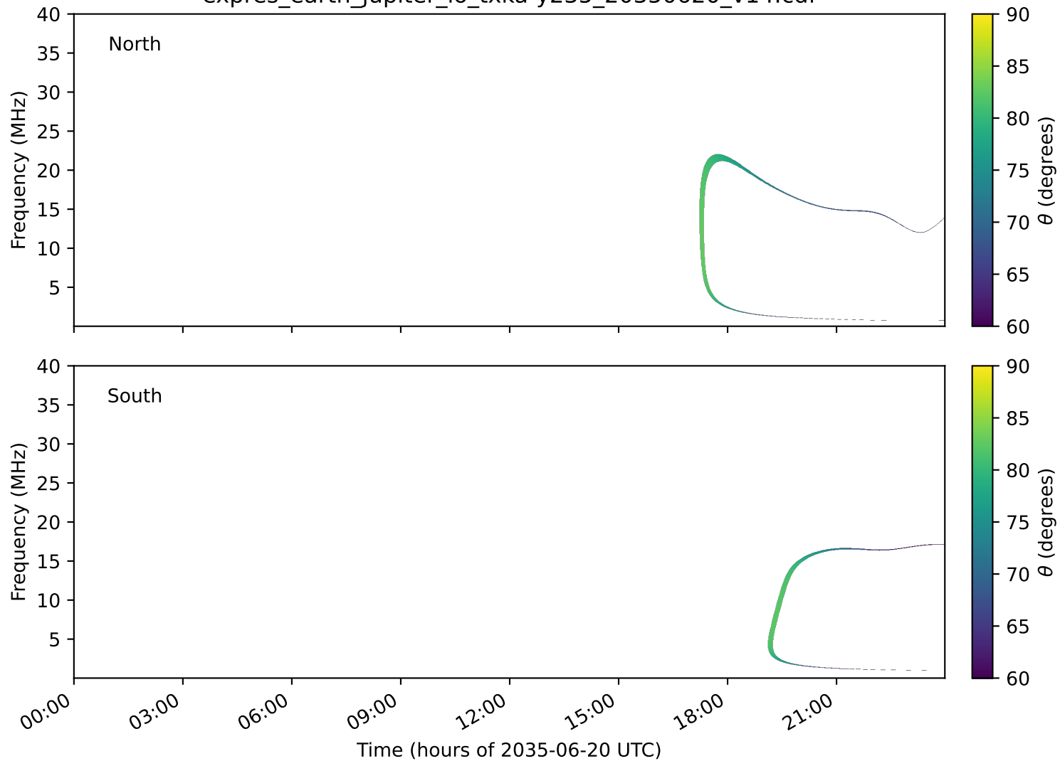
expres_earth_jupiter_io_txka-y235_20350620_v14.cdf
