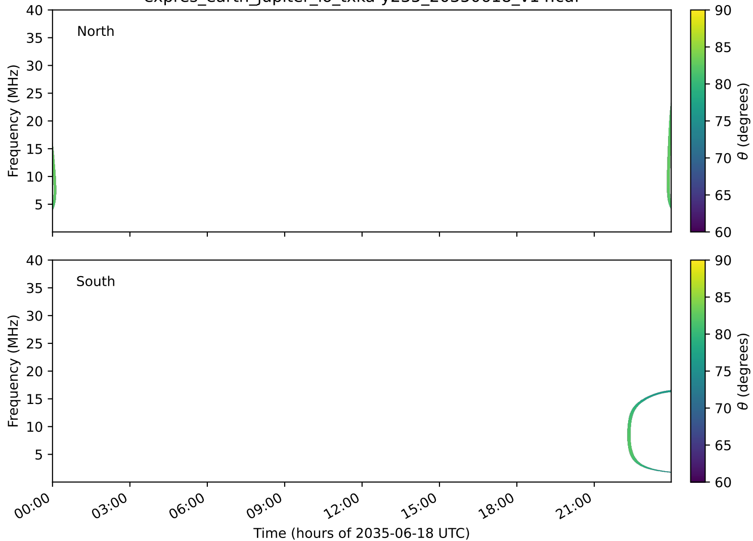
expres_earth_jupiter_io_txka-y235_20350618_v14.cdf
