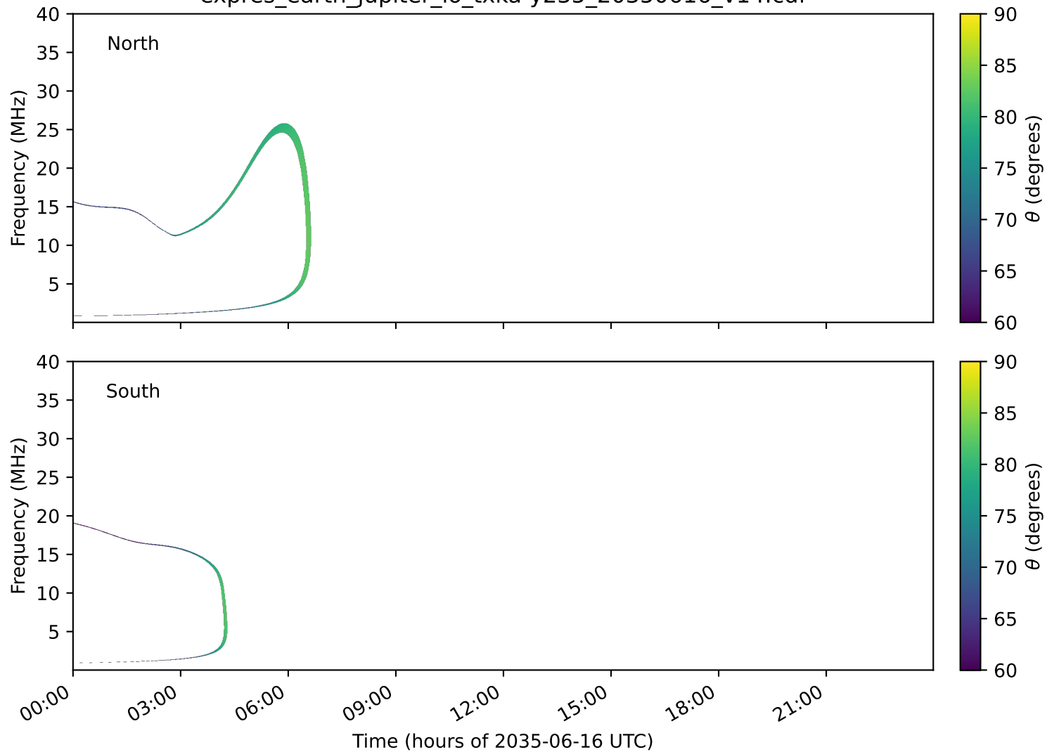
expres_earth_jupiter_io_txka-y235_20350616_v14.cdf
