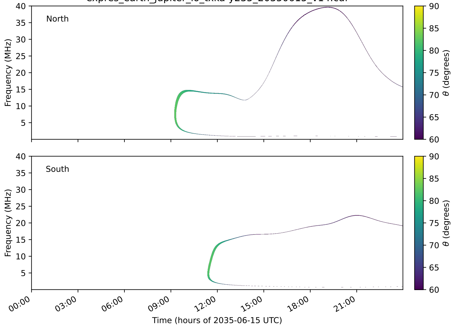
expres_earth_jupiter_io_txka-y235_20350615_v14.cdf
