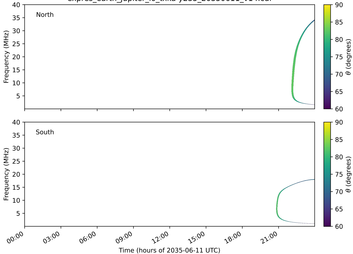
expres_earth_jupiter_io_txka-y235_20350611_v14.cdf
