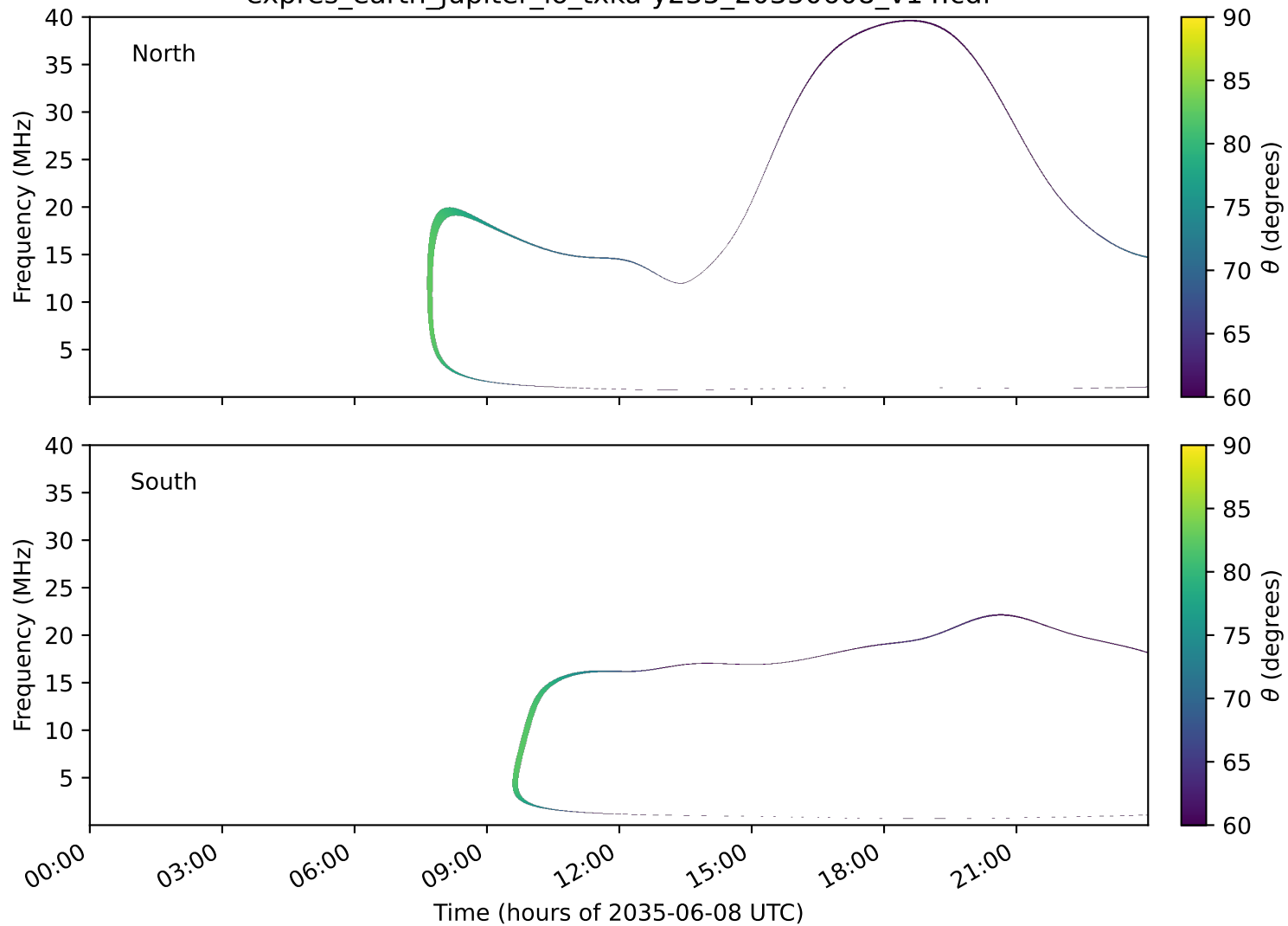
expres_earth_jupiter_io_txka-y235_20350608_v14.cdf
