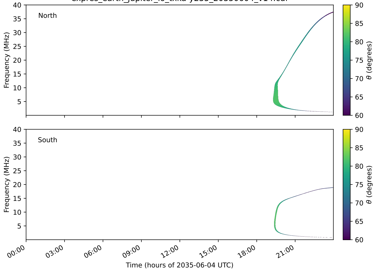
expres_earth_jupiter_io_txka-y235_20350604_v14.cdf
