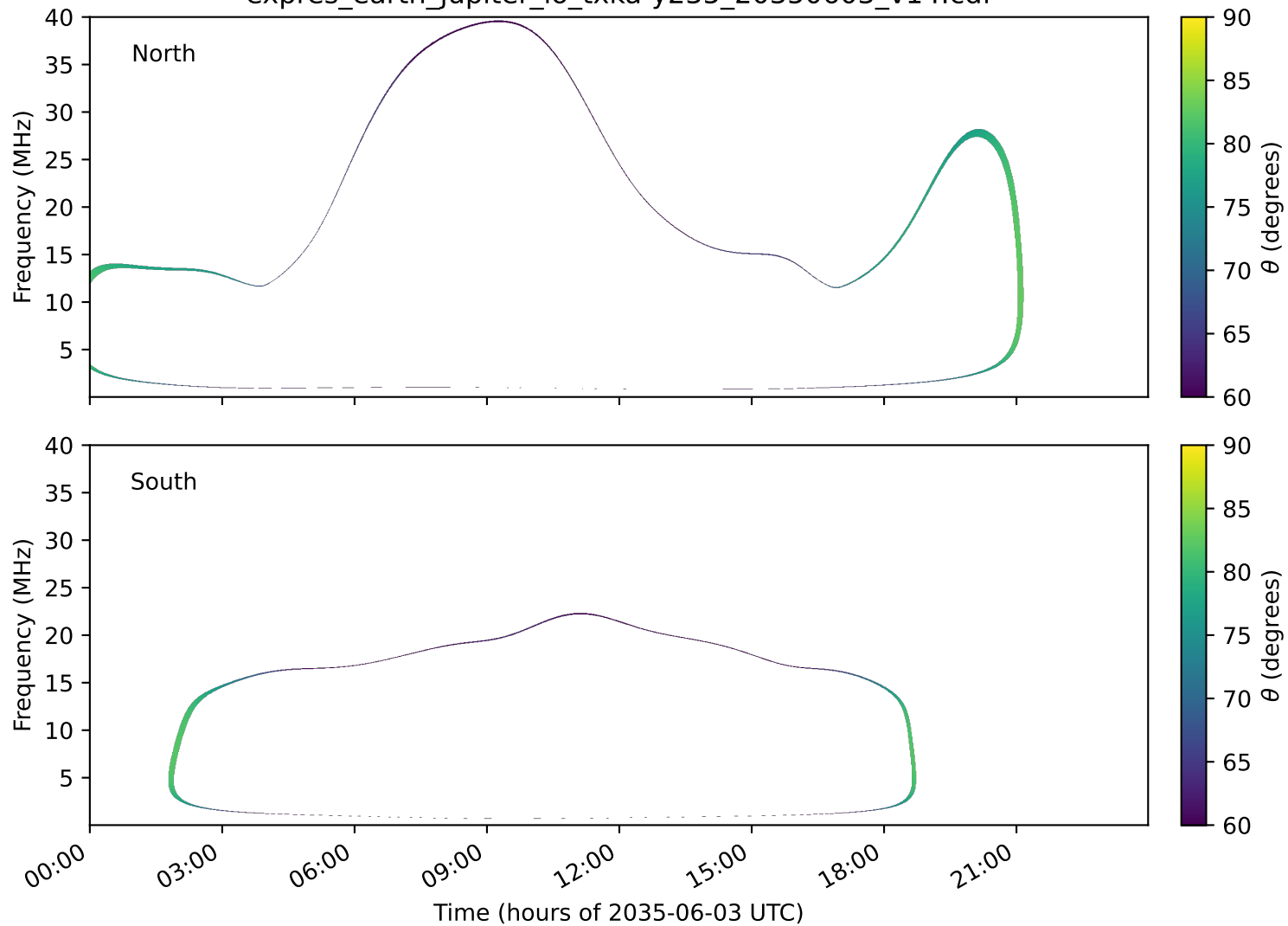
expres_earth_jupiter_io_txka-y235_20350603_v14.cdf
