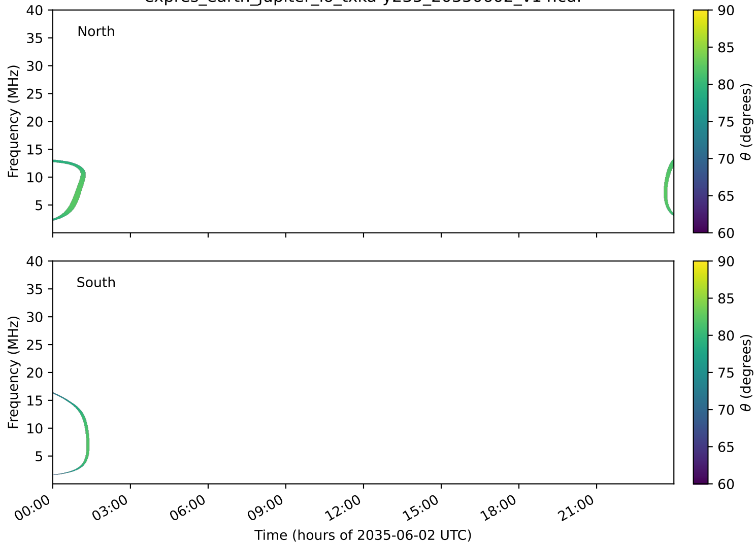
expres_earth_jupiter_io_txka-y235_20350602_v14.cdf
