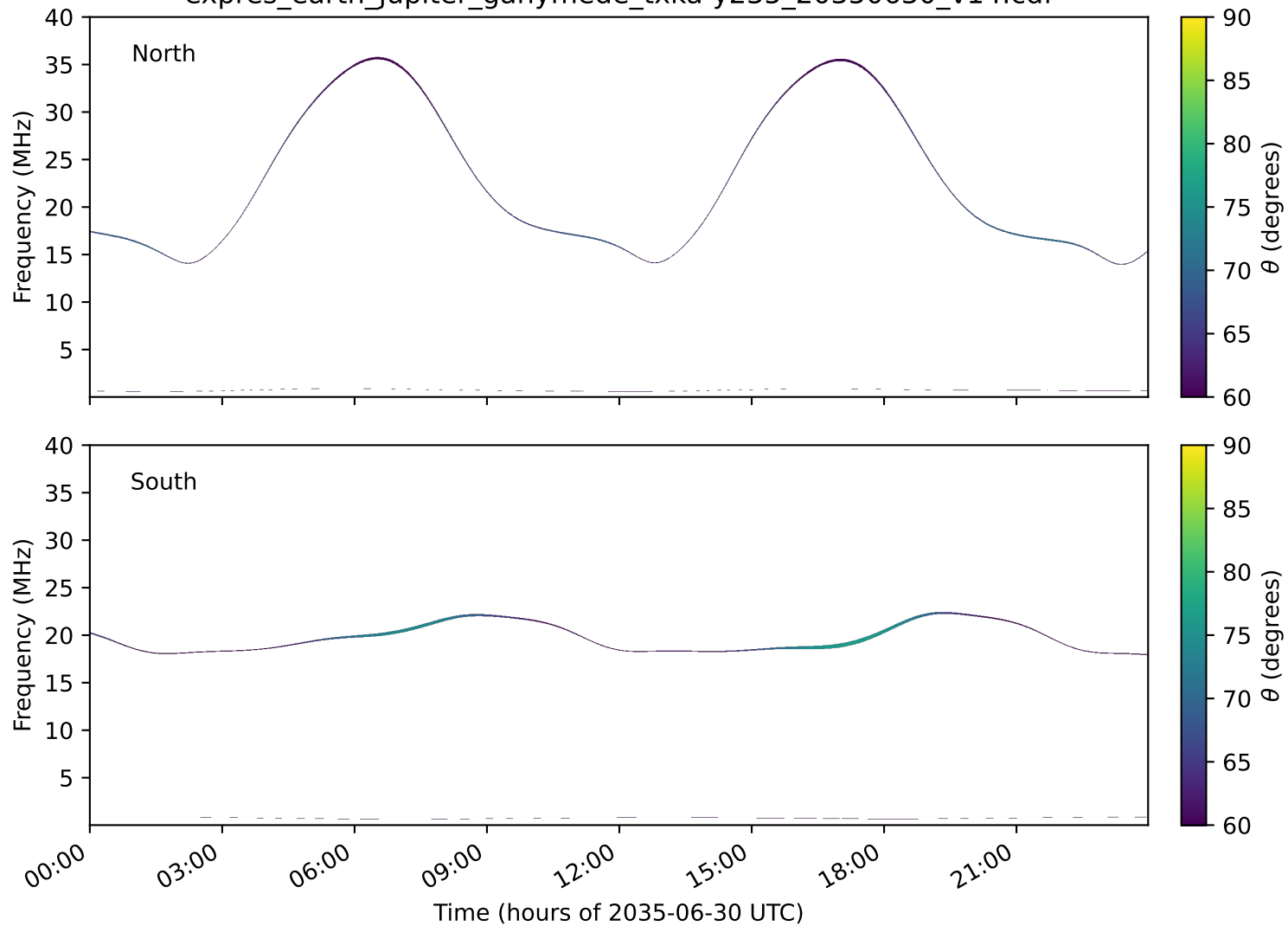
expres_earth_jupiter_ganymede_txka-y235_20350630_v14.cdf
