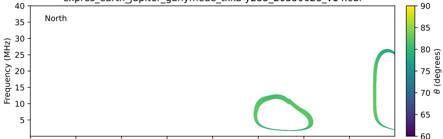
expres_earth_jupiter_ganymede_txka-y235_20350628_v14.cdf
