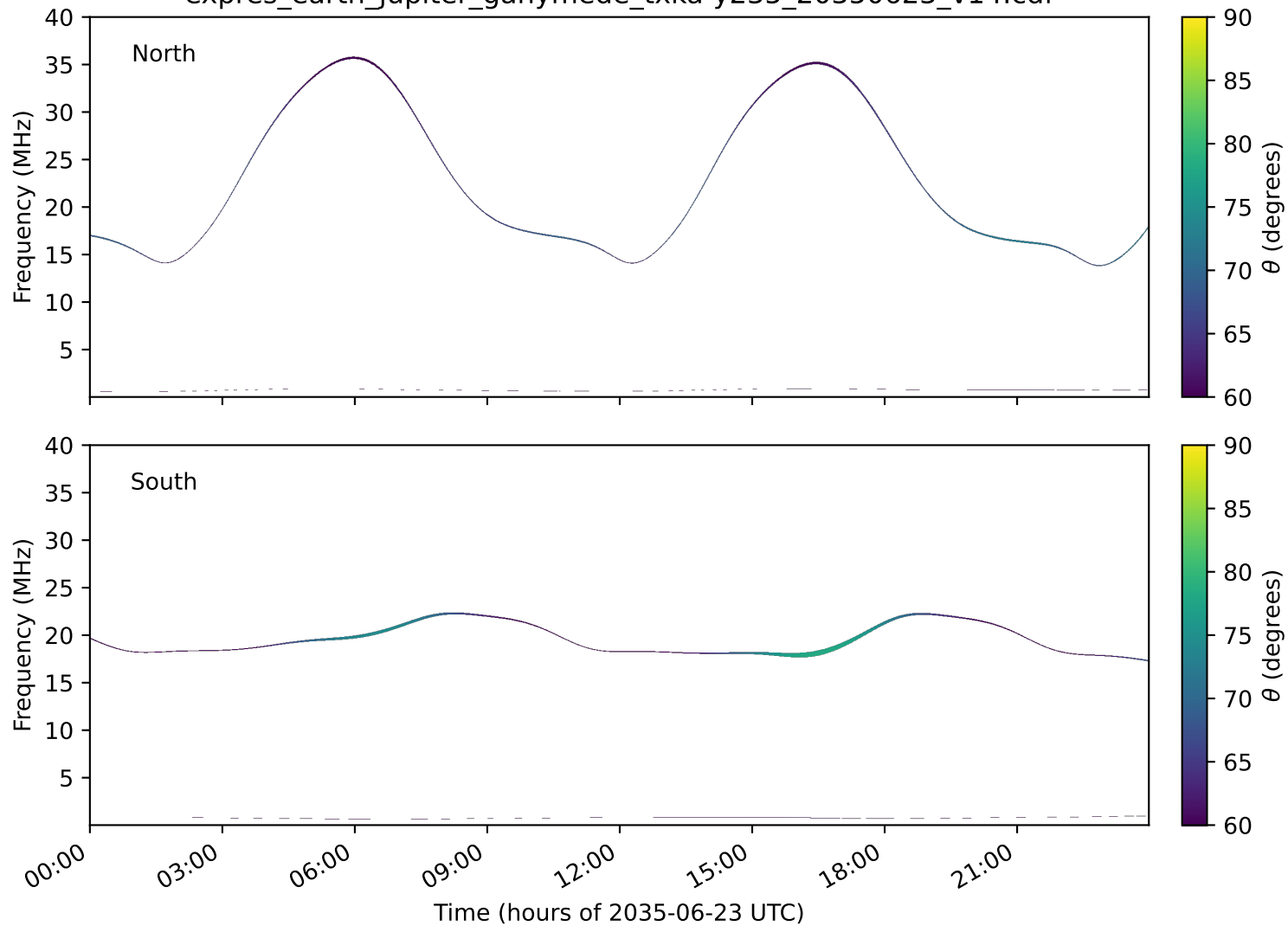
expres_earth_jupiter_ganymede_txka-y235_20350623_v14.cdf
