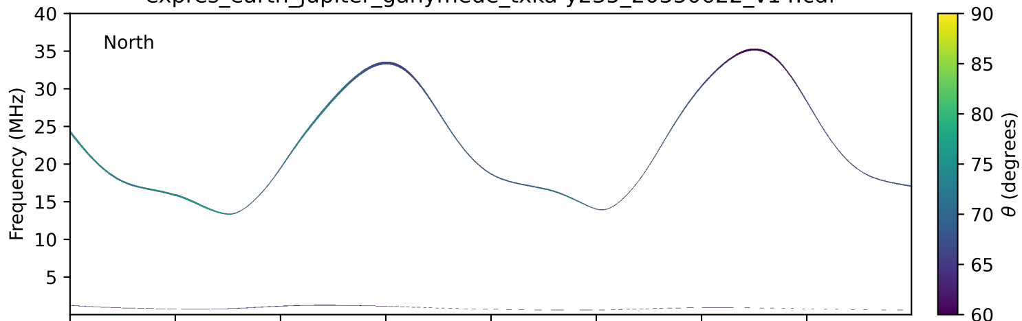
expres_earth_jupiter_ganymede_txka-y235_20350622_v14.cdf
