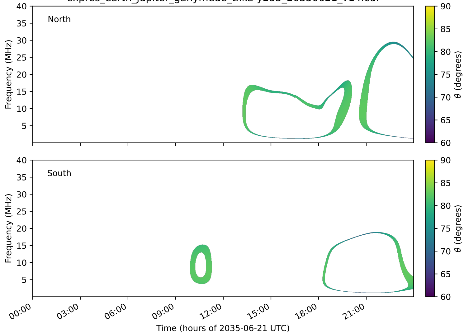
expres_earth_jupiter_ganymede_txka-y235_20350621_v14.cdf
