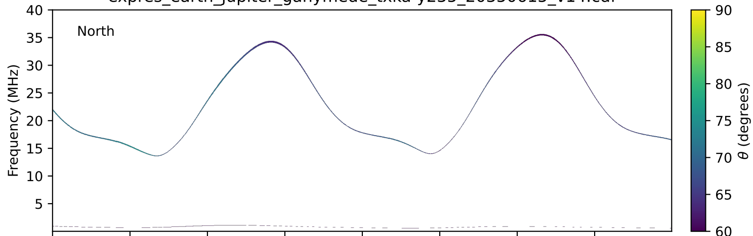
expres_earth_jupiter_ganymede_txka-y235_20350615_v14.cdf
