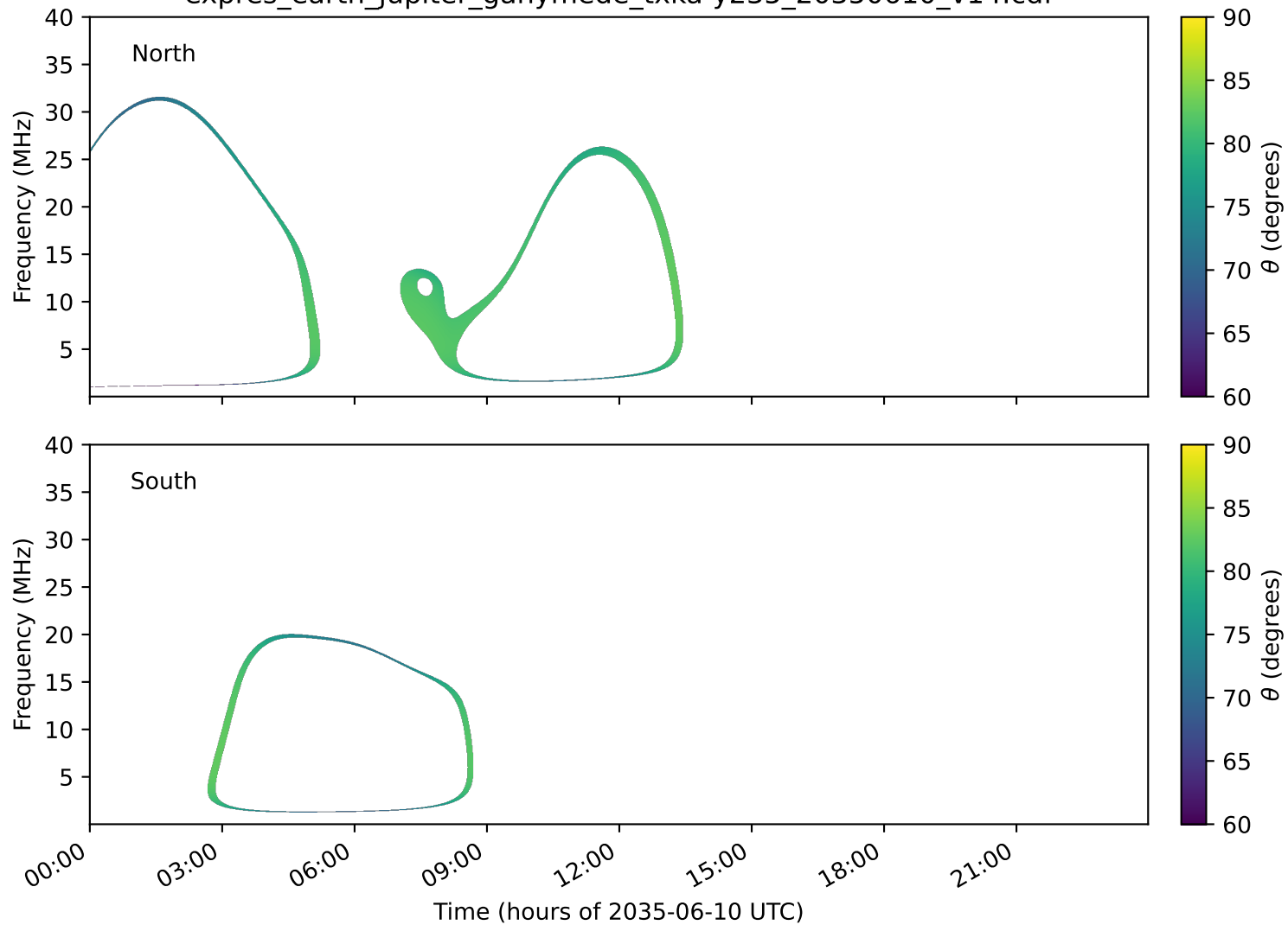
expres_earth_jupiter_ganymede_txka-y235_20350610_v14.cdf
