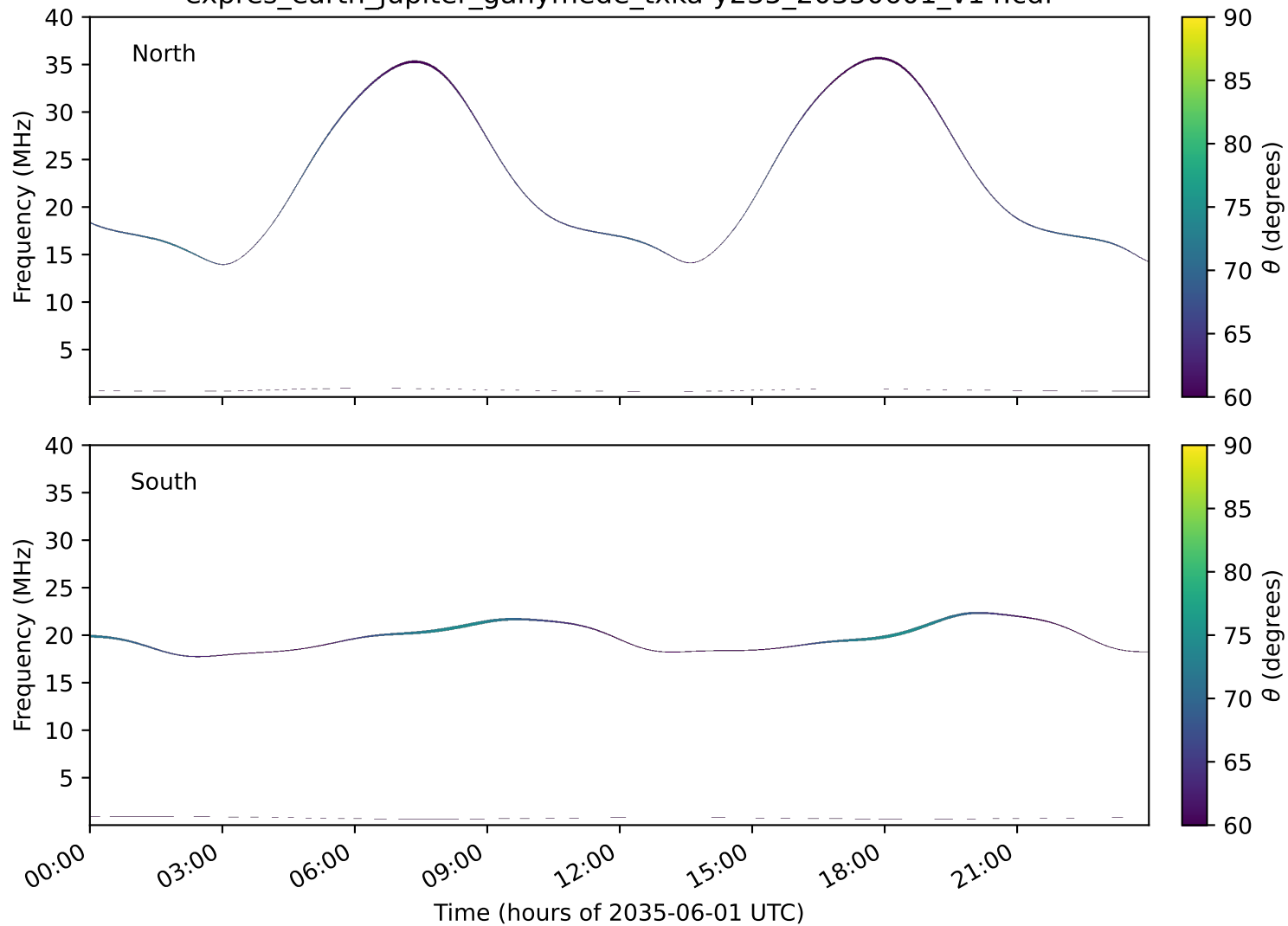
expres_earth_jupiter_ganymede_txka-y235_20350601_v14.cdf
