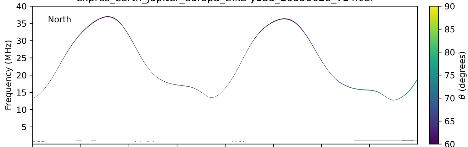
expres_earth_jupiter_europa_txka-y235_20350628_v14.cdf
