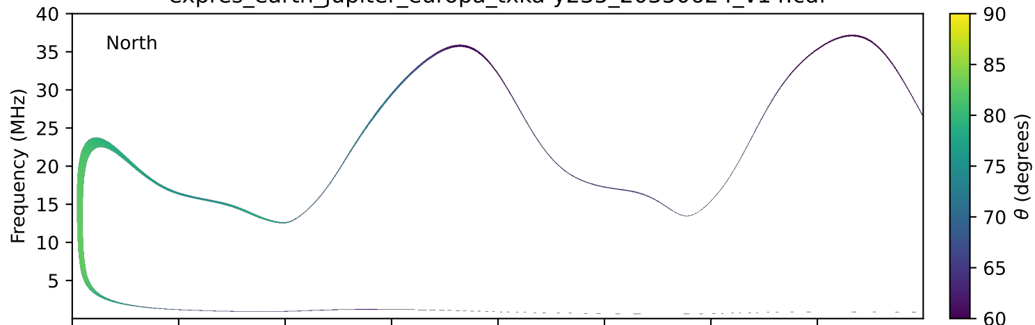
expres_earth_jupiter_europa_txka-y235_20350624_v14.cdf
