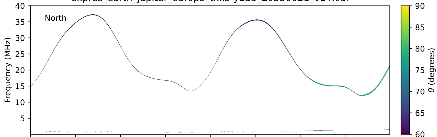
expres_earth_jupiter_europa_txka-y235_20350621_v14.cdf
