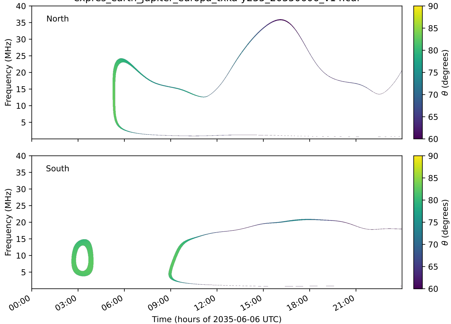
expres_earth_jupiter_europa_txka-y235_20350606_v14.cdf
