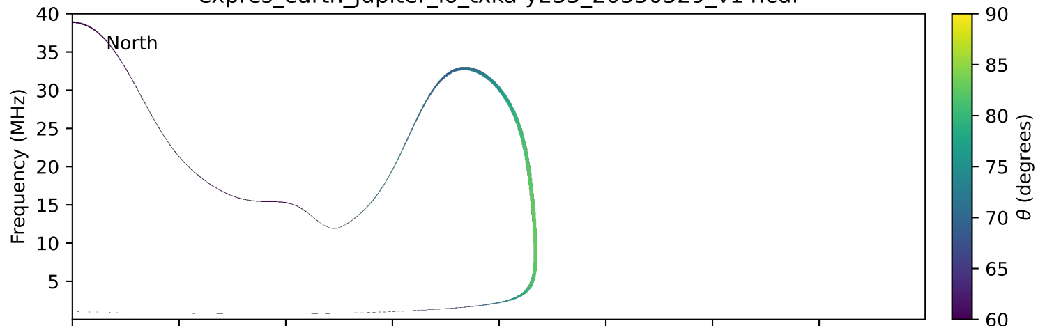
expres_earth_jupiter_io_txka-y235_20350529_v14.cdf
