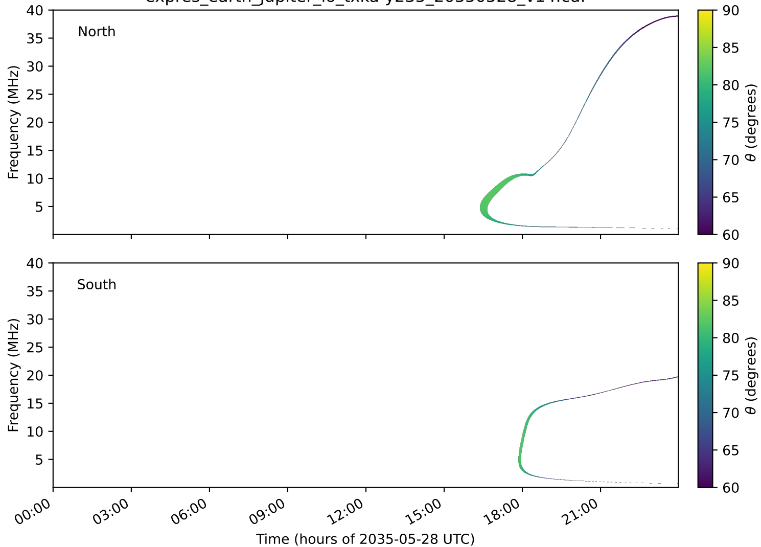
expres_earth_jupiter_io_txka-y235_20350528_v14.cdf
