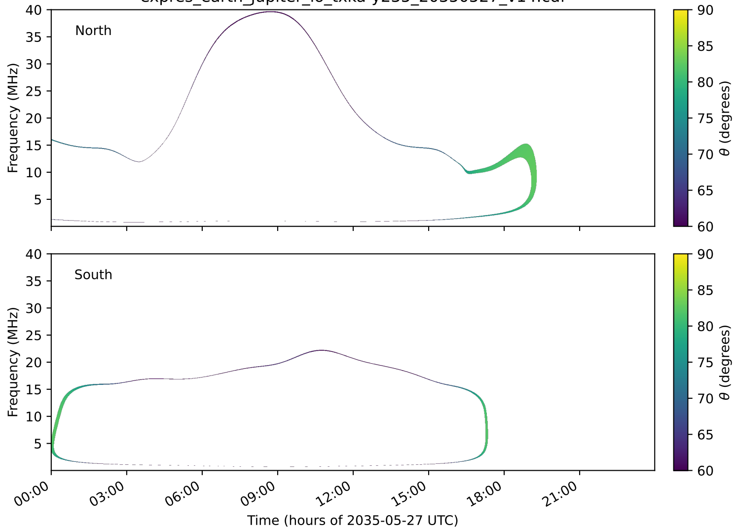
expres_earth_jupiter_io_txka-y235_20350527_v14.cdf
