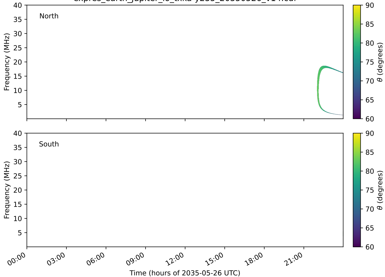
expres_earth_jupiter_io_txka-y235_20350526_v14.cdf
