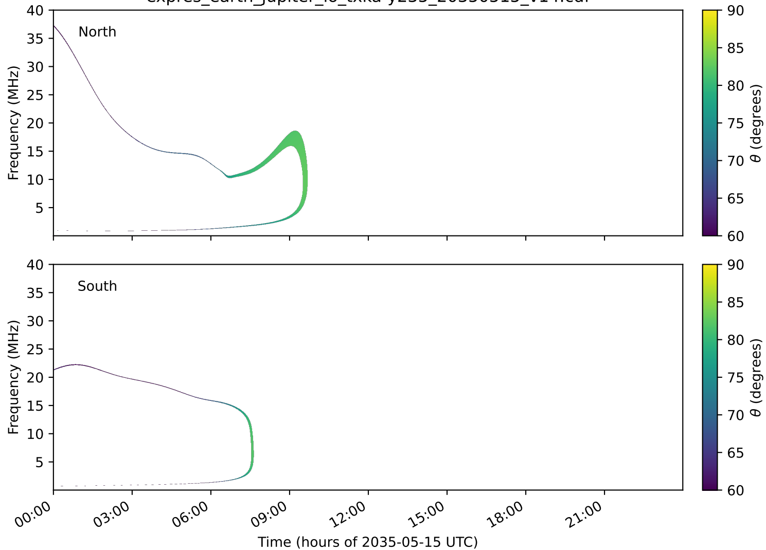
expres_earth_jupiter_io_txka-y235_20350515_v14.cdf
