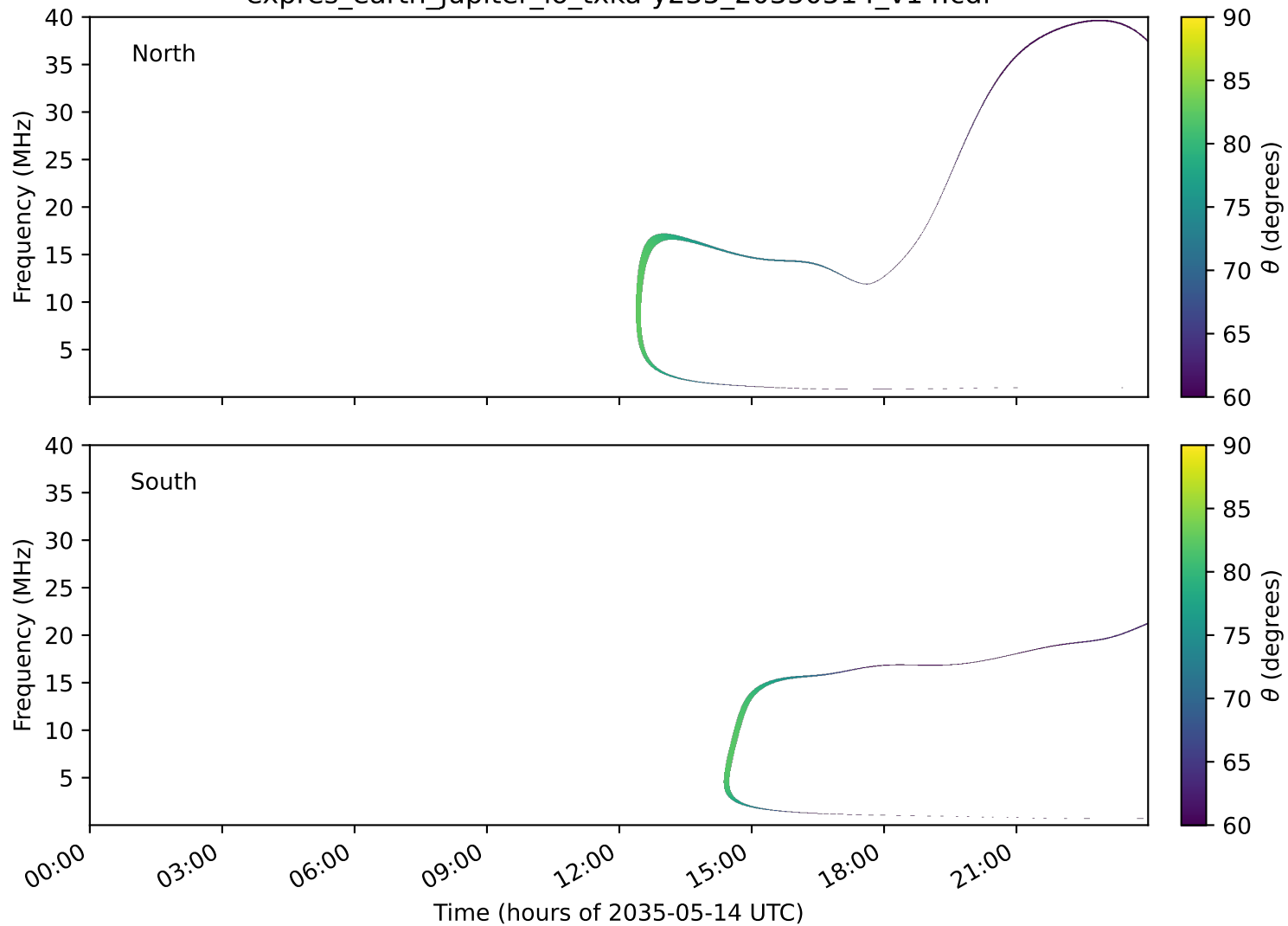
expres_earth_jupiter_io_txka-y235_20350514_v14.cdf
