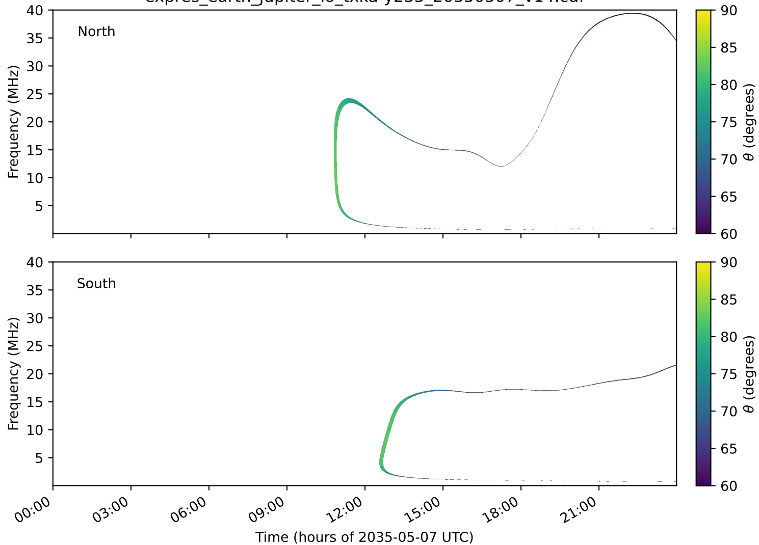
expres_earth_jupiter_io_txka-y235_20350507_v14.cdf
