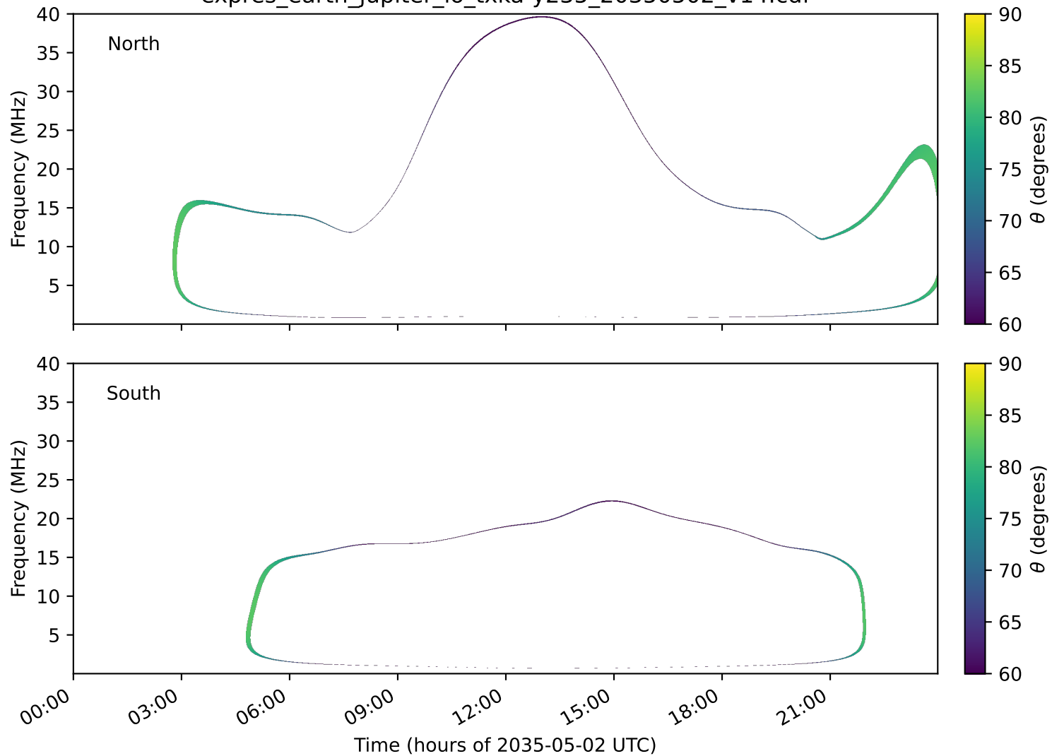
expres_earth_jupiter_io_txka-y235_20350502_v14.cdf
