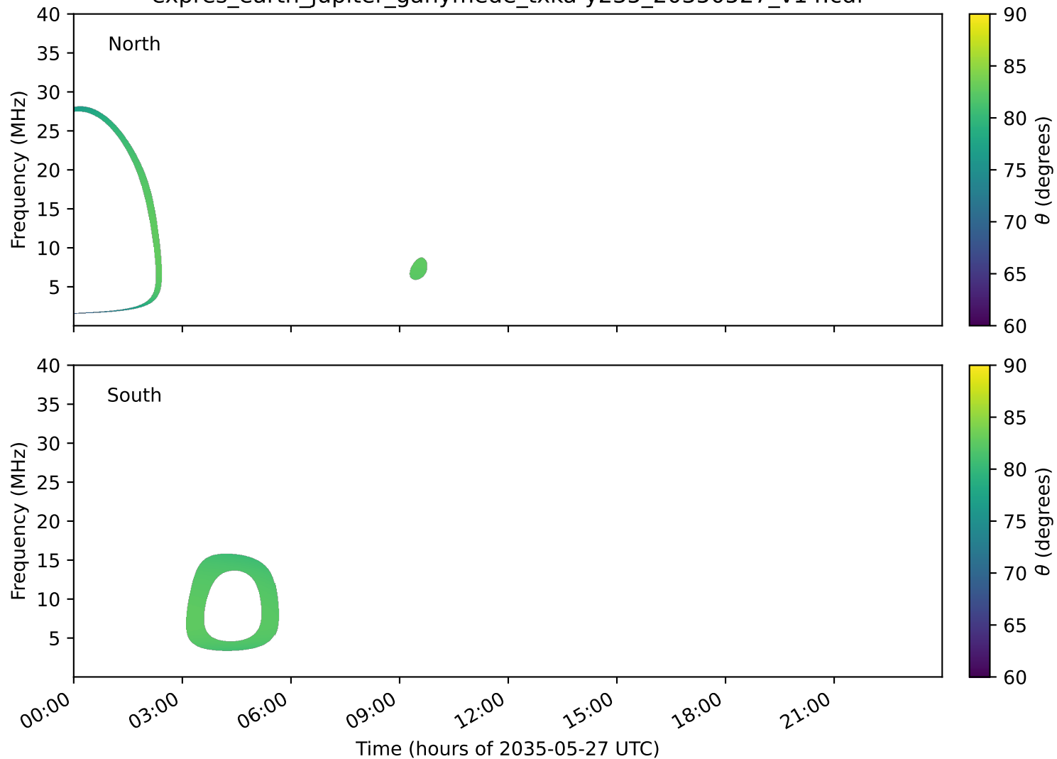
expres_earth_jupiter_ganymede_txka-y235_20350527_v14.cdf
