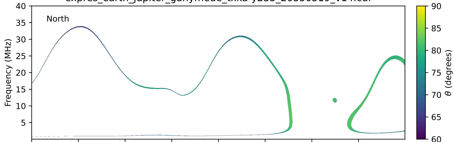
expres_earth_jupiter_ganymede_txka-y235_20350519_v14.cdf
